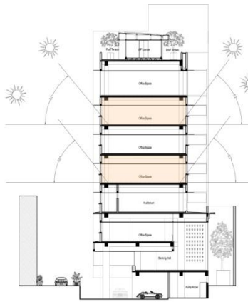
Figure 31, the sectional form of CDB. It can be seen that solar angles lower than 53^{\circ} in altitude results in direct solar radiation exposure of the typical office floors. Much lower angles does not affect the building due to the tight urban context.
