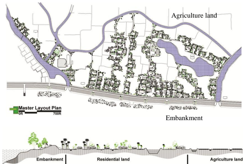
Fig 09: Proposed Plan and section, Gabura Union (7 no.ward), Source: Author
